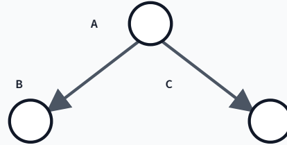
Common cause
