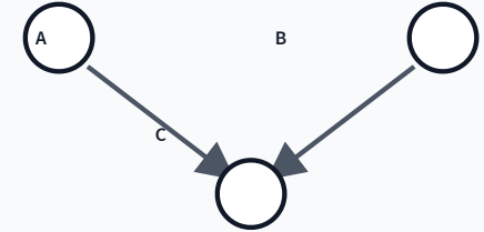
V-structure
