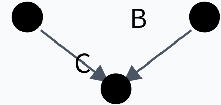
V-structure
