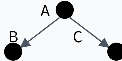
Common cause
