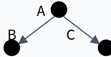
Common cause
