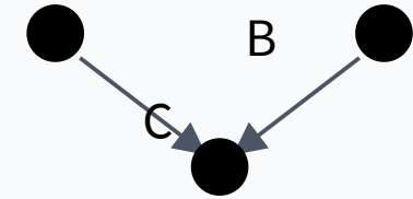
V-structure
