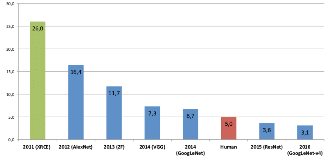
ImageNet Classification Error (Top 5)
