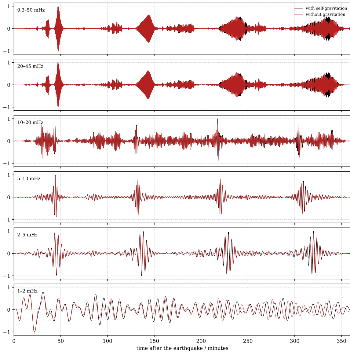
Fig. 2: Synthetic vertical-component acceleration seismograms in the earth model PREM for an earthquake of moment magnitude 8 at 20 km depth, recorded at an epicentral angle of 90°, computed with (black) and without (red) self-gravitation. The top trace shows the full band of the calculation, from 0.3 to 50 mHz, and those below it the same seismogram band-pass filtered in successively lower frequency bands. Each trace is normalised by its maximum. The calculations neglect attenuation, so that the surface waves continue to circle the Earth undiminished over the six hours shown. The two calculations differ only in the lowest bands, and there the differences grow with time as the long-period surface waves circle the Earth.
