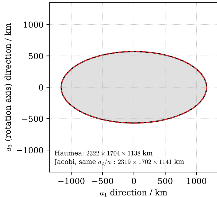
meridional section
