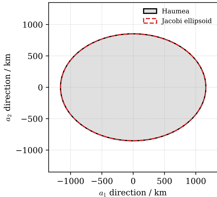
equatorial section
