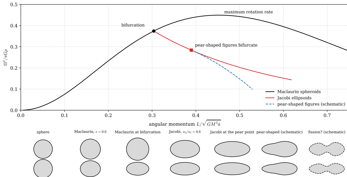
Fig. 3: The Maclaurin and Jacobi sequences of equilibrium figures of a homogeneous rotating fluid, shown as the dimensionless rotation rate \Omega^2/\pi G\rho against the dimensionless angular momentum, where \bar{a} is the mean radius. The Jacobi sequence branches from the Maclaurin sequence at the point marked, and the pear-shaped figures of Poincaré branch from the Jacobi sequence at the square. The pear-shaped sequence is known only approximately and is drawn schematically; its figures are unstable. Below are the equatorial (upper) and meridional (lower) sections of some members of the sequences, all with the same volume, followed by sketches of a pear-shaped figure and of the fissioning figure that was once imagined to lie beyond it; no closed form exists for these, and the sketches are only schematic.
