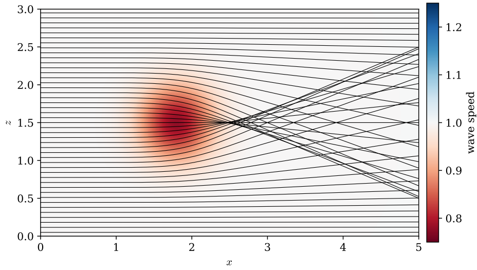
Fig. 3: Rays from an initially plane wavefront passing through a smooth region of low wave speed, obtained by numerical integration of Hamilton's equations. Behind the anomaly the rays cross, and their envelope forms a caustic.
