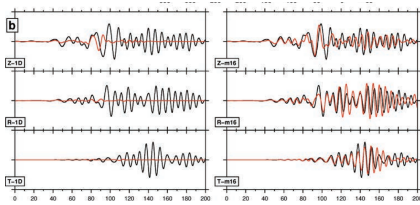
Fig. 2: An example of observed and synthetic three-component seismograms from a waveform tomographic study of Southern California. Data are shown in black, and synthetics in red. On the left the comparison is made prior to inversion, with the synthetics calculated in a laterally homogeneous model. The right-hand side then shows the data fit following inversion involving 16 iterative model updates. Taken from Tape et al. (2010).
