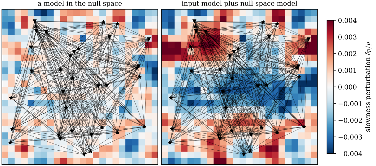
Fig. 3: A model lying in the null space of the toy tomographic problem shown in Fig. 2 (left), and the input model of that figure with this null-space model added (right). The two models on the right of Fig. 2 and here produce identical delay times along every ray, and so cannot be distinguished by the data.
