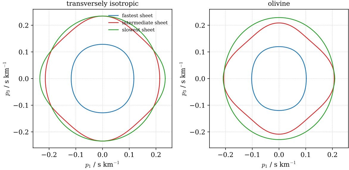
Fig. 1: Plane sections through the slowness surfaces of two anisotropic materials, calculated numerically from the Christoffel equation. On the left is a transversely isotropic medium, with the section containing the symmetry axis (which is vertical); on the right is a single crystal of olivine, an orthorhombic mineral that makes up much of the upper mantle, using the elastic constants of Abramson et al. (1997). The three sheets of the slowness surface are shown in different colours, and there are directions along which two of the sheets touch.
