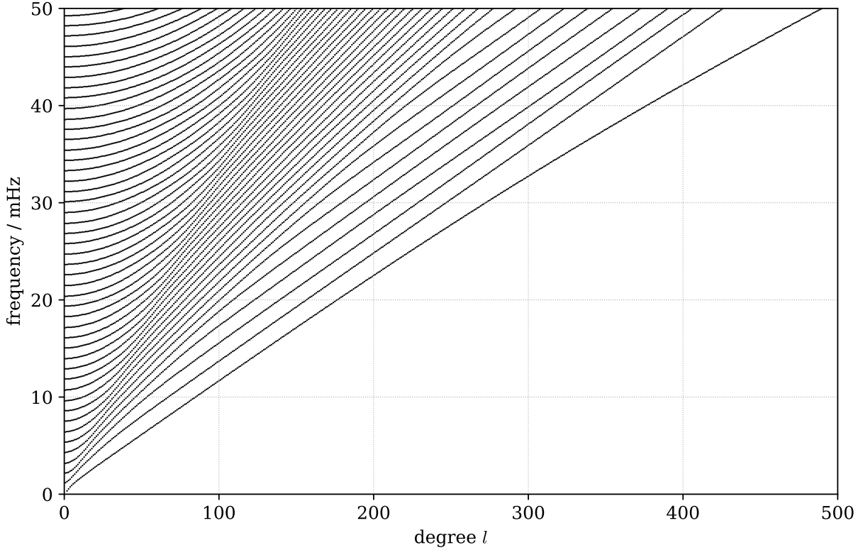
Fig. 1: Eigenfrequencies of toroidal modes within the earth model PREM of Dziewonski & Anderson (1981), plotted against degree l for frequencies up to 50 mHz. For each degree we see a set of different overtones that can be labelled using the overtone number n , the lowest curve being the fundamental branch n = 0 . Note also that PREM comprises a solid inner core, fluid outer core, and solid mantle and crust. The modes seen here are mantle toroidal modes, but one could also calculate toroidal modes confined to the inner core.
