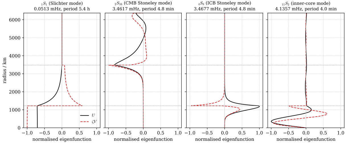
Fig. 4: Radial eigenfunctions of some less typical spheroidal modes of PREM: the Slichter mode {}_1S_1 , in which the inner core translates within the fluid outer core; Stoneley modes trapped on the core–mantle boundary and on the inner-core boundary; and a mode confined almost entirely to the inner core.
