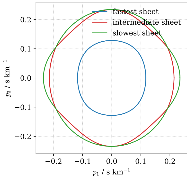
transversely isotropic
