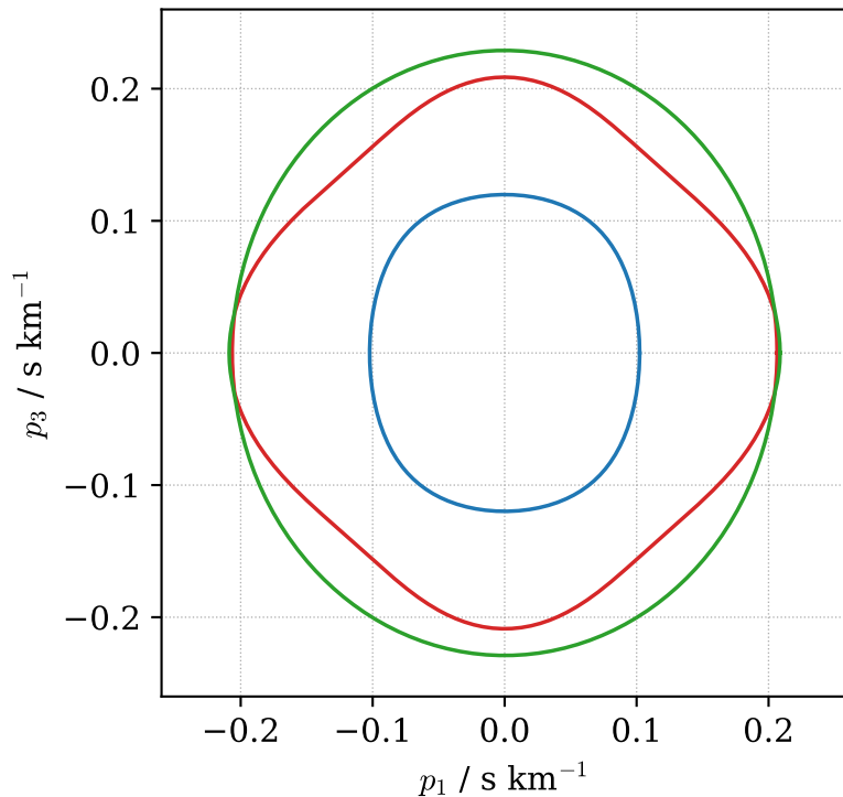
olivine
