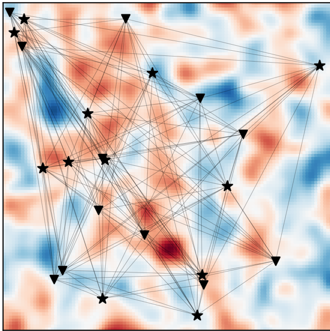
true model
