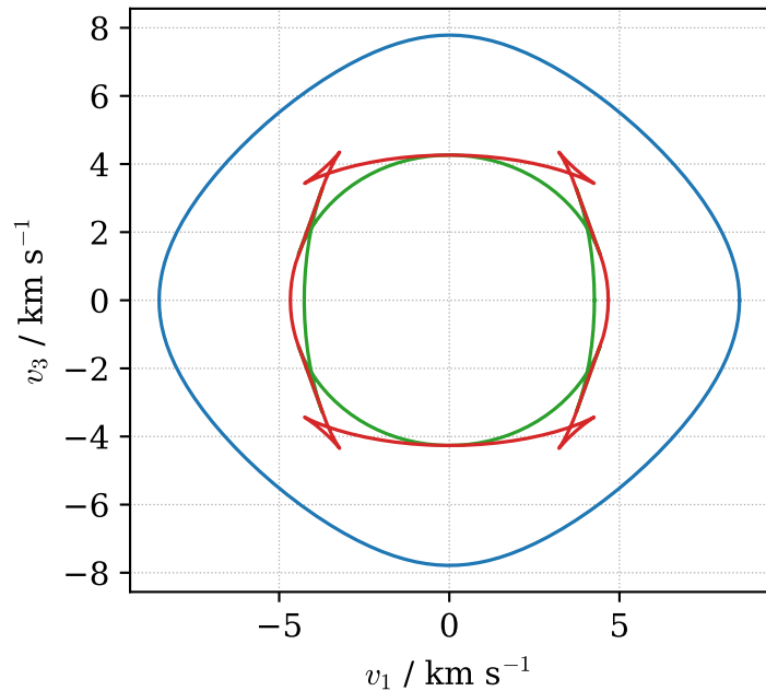
wave surface
