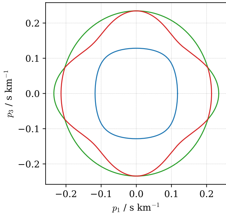
slowness surface
