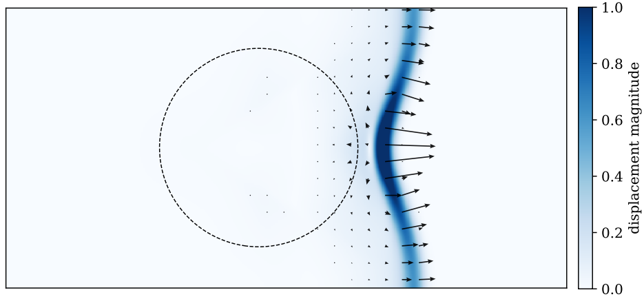
Fig. 2: As for Fig. 1, but for the passage of a plane P-wave through a heterogeneous region having length scale much larger than that of the incident wave. Here we see minimal scattering, along with the smooth distortion of the wavefront and associated amplitude and polarisation variations. This is a situation to which ray theory can be usefully applied.
