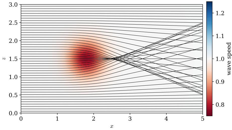
Fig. 3: Rays from an initially plane wavefront passing through a smooth region of low wave speed, obtained by numerical integration of Hamilton's equations. Behind the anomaly the rays cross, and their envelope forms a caustic.
