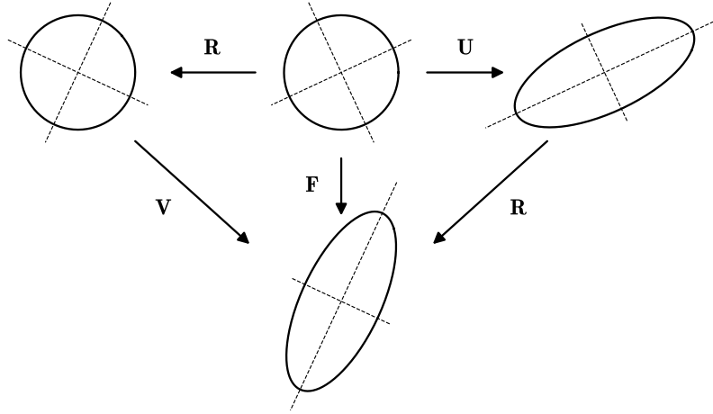
Fig. 1: Under an invertible matrix \mathbf{F} , a circle (in three dimensions, a sphere) is mapped to an ellipse (ellipsoid). Using this fact, the geometric meaning of the polar decomposition theorem is shown. An undeformed circle is shown in the centre of the upper row, with the dashed lines along the eigenvectors of the symmetric matrix \mathbf{U} ; in the other panels the dashed lines show the images of these axes.
