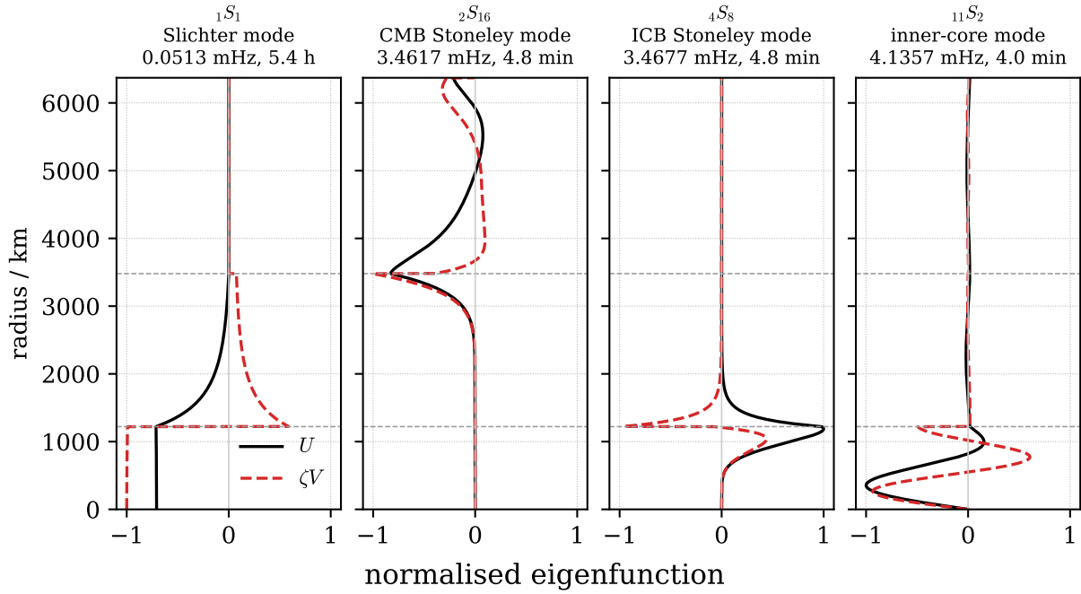
Fig. 4: Radial eigenfunctions of some less typical spheroidal modes of PREM: the Slichter mode {}_1S_1 , in which the inner core translates within the fluid outer core; Stoneley modes trapped on the core–mantle boundary and on the inner-core boundary; and a mode confined almost entirely to the inner core.
