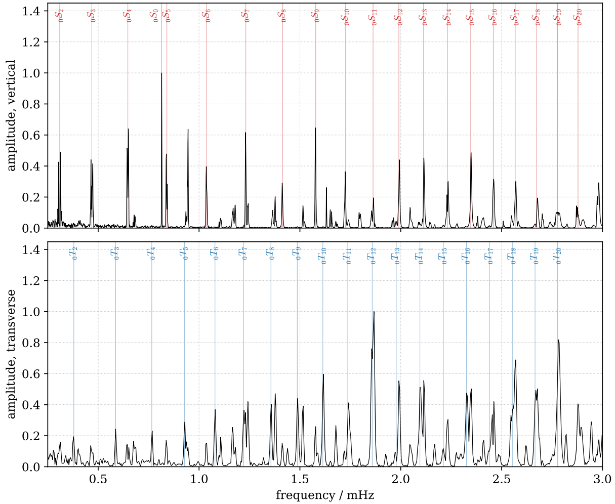
Fig. 2: Amplitude spectra of the record in Fig. 1. The upper panel is for the full ten days of the vertical component, and the lower panel for the first three days of the transverse horizontal component (perpendicular to the great circle from the earthquake), a shorter window being used because horizontal records are noisier at low frequencies. The vertical lines mark the frequencies of the fundamental spheroidal modes {}_0S_l (upper panel) and toroidal modes {}_0T_l (lower panel) in the earth model PREM; the largest peak in the upper panel is the radial mode {}_0S_0 , and most of the unlabelled peaks are overtones. In some cases individual mode peaks can be identified, but at higher frequencies there is substantial overlap of the peaks due both to attenuation and an insufficiently long time series. The lowest-frequency peaks are also visibly split into several closely spaced peaks, an effect of the Earth's rotation and asphericity that we return to in the next lecture.
