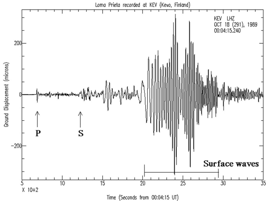
Fig. 2: A vertical component seismogram recorded in Finland following an earthquake in California (the 1989 Loma Prieta earthquake recorded at station KEV). The P-wave arrival can be seen very clearly, while later arriving phases are significantly harder to identify.
