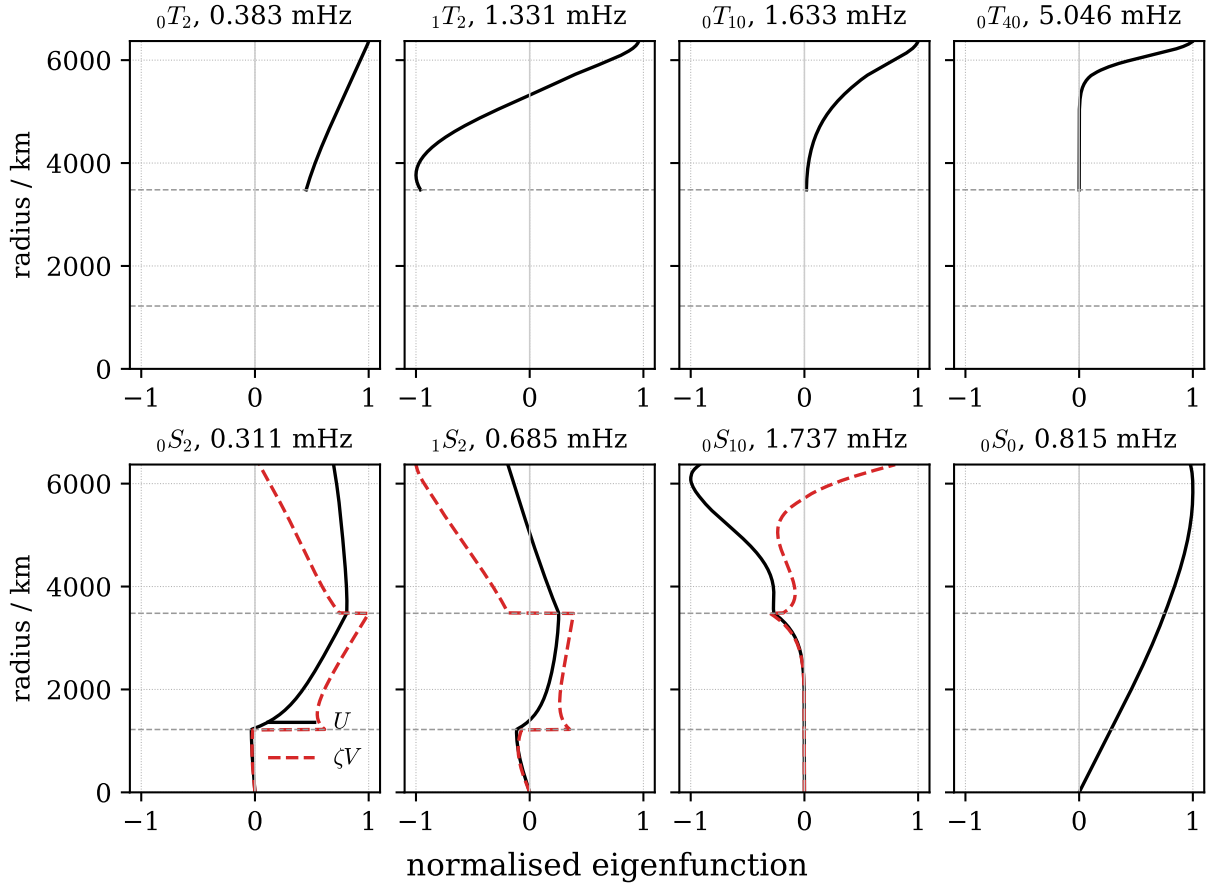
Fig. 3: Radial eigenfunctions of some toroidal (upper row) and spheroidal (lower row) modes of PREM, each normalised to unit maximum amplitude. For the spheroidal modes both the radial component U and the tangential component \zeta V , where \zeta = \sqrt{l(l+1)} , are shown. The dashed lines mark the core–mantle and inner-core boundaries. Calculated using the spectral-element normal-mode code of A. Myhill.
