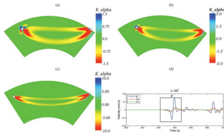
Fig. 5: Cross-sections through the functional derivative of a cross-correlation delay time for a P-wave phase with respect to \alpha as calculated by the adjoint method. The delay time of the same phase can be measured at different frequencies by filtering the data and synthetic waveforms: panels (a)–(c) show the kernel for three different period bands, each on its own colour scale, and (d) the filtered synthetic seismograms at an epicentral distance of 60^\circ , with the box marking the window around the P arrival used for the measurement. The dominant sensitivity lies within the first Fresnel zone, but it curiously vanishes along the ray path. Figure taken from Liu & Tromp (2008).
