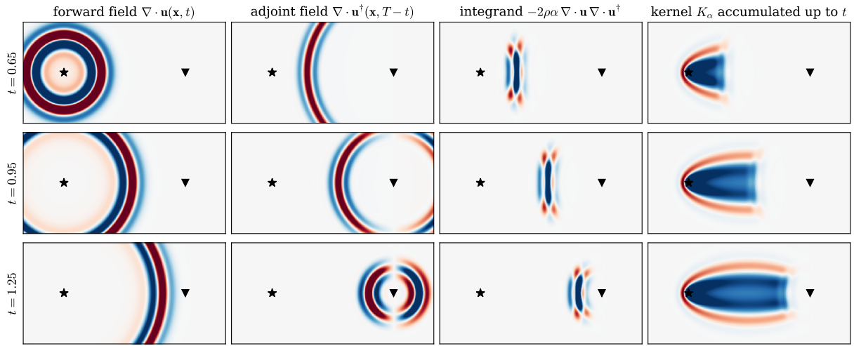
Fig. 3: Construction of a cross-correlation delay-time kernel by the adjoint method in a two-dimensional homogeneous body. The star marks an explosive source and the triangle a receiver. The kernel is K_\alpha(\mathbf{x}) = -2\rho\alpha \int_0^T \nabla \cdot \mathbf{u}(\mathbf{x}, t) \nabla \cdot \mathbf{u}^\dagger(\mathbf{x}, T - t) dt , and each row shows one instant t (times are in nondimensional units, with T \approx 2 ): the divergence of the forward field \mathbf{u}(\mathbf{x}, t) ; the divergence of the adjoint field \mathbf{u}^\dagger(\mathbf{x}, T - t) after it has evolved for a time T - t from the receiver; the integrand, that is the instantaneous contribution to the kernel; and the kernel accumulated over times up to t . The integrand, and hence the kernel, is non-zero only where the two fields overlap.
