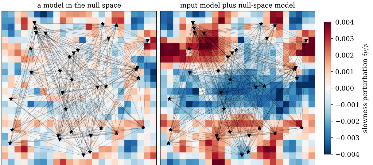
Fig. 3: A model lying in the null space of the toy tomographic problem shown in Fig. 2 (left), and the input model of that figure with this null-space model added (right). The input model on the left of Fig. 2 and the model on the right here produce identical delay times along every ray, and so cannot be distinguished by the data.
