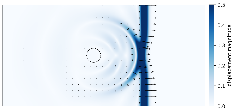
Fig. 1: Snapshot from a numerical simulation of the scattering of a plane P-wave in a homogeneous background model due to its interaction with a heterogeneity having a typical length scale approximately equal to the length scale of the incident wave. The colours show the magnitude of the displacement, the arrows show the particle motion, and the dashed line marks the extent of the heterogeneity; the colour scale is saturated so as to show the weak scattered field. The box is about 13 wavelengths of the incident wave wide and 6 high. We see that the scattered wavefield comprises both P-waves and S-waves.
