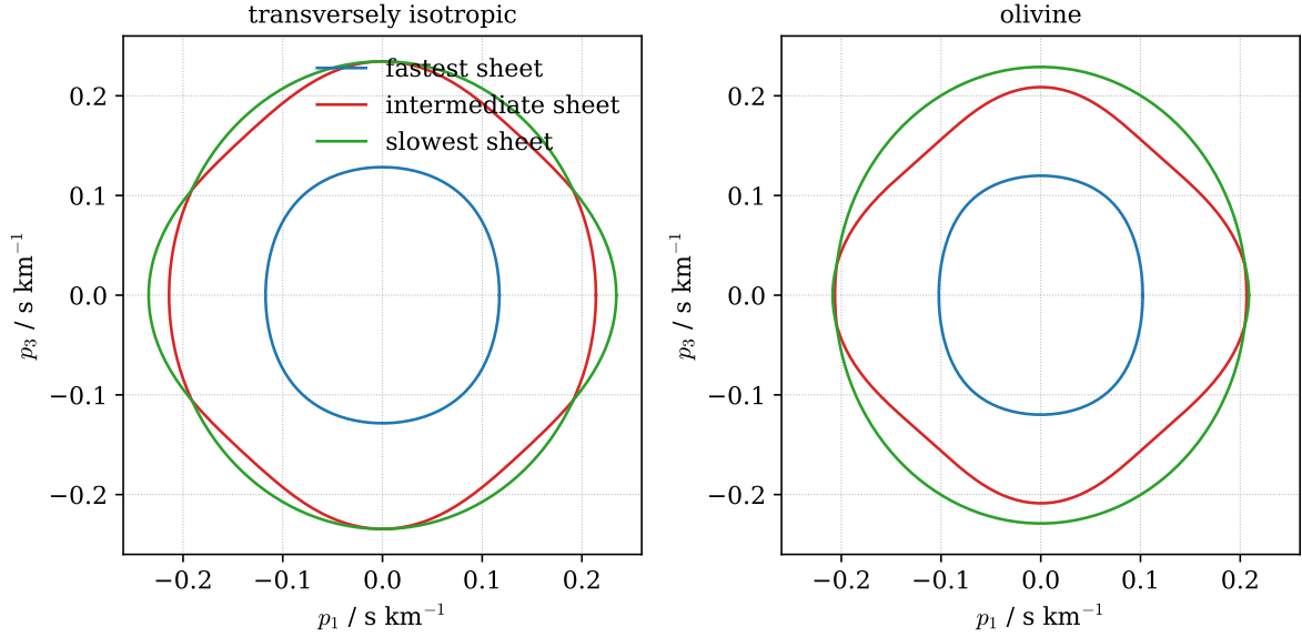
Fig. 1: Plane sections through the slowness surfaces of two anisotropic materials, calculated numerically from the Christoffel equation. On the left is a transversely isotropic medium with Love moduli A = 240 , C = 200 , F = 70 , L = 60 and N = 72 GPa and density 3300 \text{ kg m}^{-3} , with the section containing the symmetry axis (which is vertical); on the right is a single crystal of olivine (section in the [100] – [001] plane), an orthorhombic mineral that makes up much of the upper mantle, using the elastic constants of Abramson et al. (1997). The three sheets of the slowness surface are shown in different colours, and there are directions along which two of the sheets touch.
