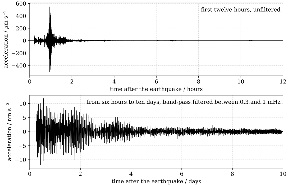
Fig. 1: Vertical-component acceleration recorded at the Black Forest Observatory in Germany following the 2011 Tohoku earthquake in Japan (moment magnitude 9.1). The upper panel shows the first twelve hours of the record, dominated by the surface waves, which circle the Earth several times. The lower panel shows the record from six hours to ten days after the earthquake, band-pass filtered between 0.3 and 1 mHz to isolate the lowest-frequency free oscillations. Their amplitude decays in a roughly exponential fashion over several days. This decay is due to attenuation within the Earth, but we ignore this effect within our current discussion.
