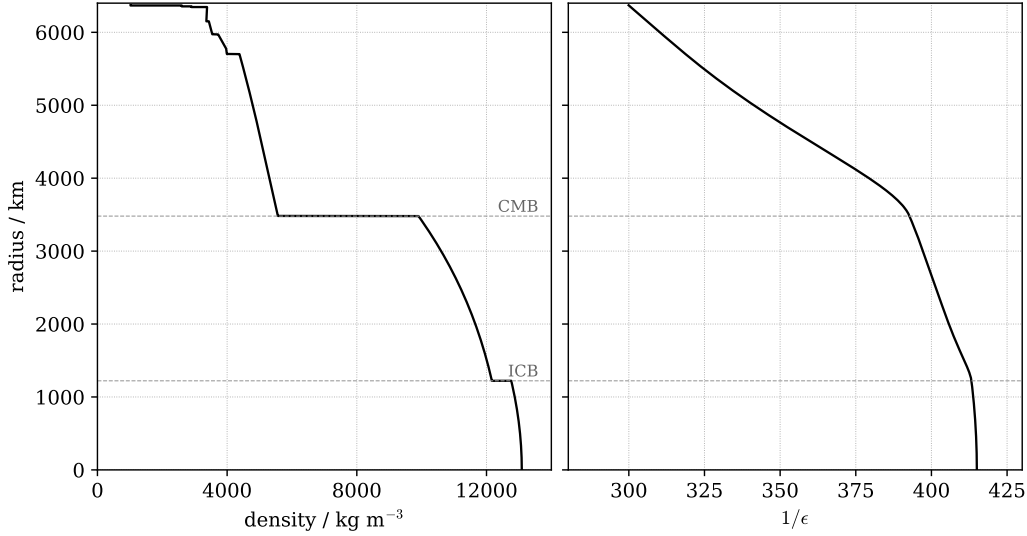
Fig. 2: Left: the Earth's spherically averaged density according to the model PREM, which was determined from free oscillation data along with the mass and moment of inertia. Right: the reciprocal of the ellipticity obtained by numerical solution of Clairaut's equation for this density profile. At the surface 1/\epsilon \approx 300 , while at the centre it is about 415.
