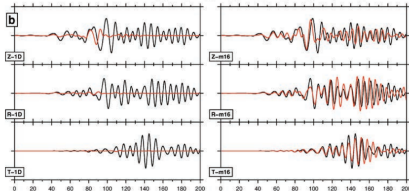
Fig. 2: An example of observed and synthetic three-component seismograms from a waveform tomographic study of Southern California. Data are shown in black, and synthetics in red; the rows show the vertical (Z), radial (R) and transverse (T) components, and time is in seconds. On the left (1D) the comparison is made prior to inversion, with the synthetics calculated in the initial, laterally homogeneous, model. The right-hand side (m16) then shows the data fit following inversion involving 16 iterative model updates. Taken from Tape et al. (2010).
