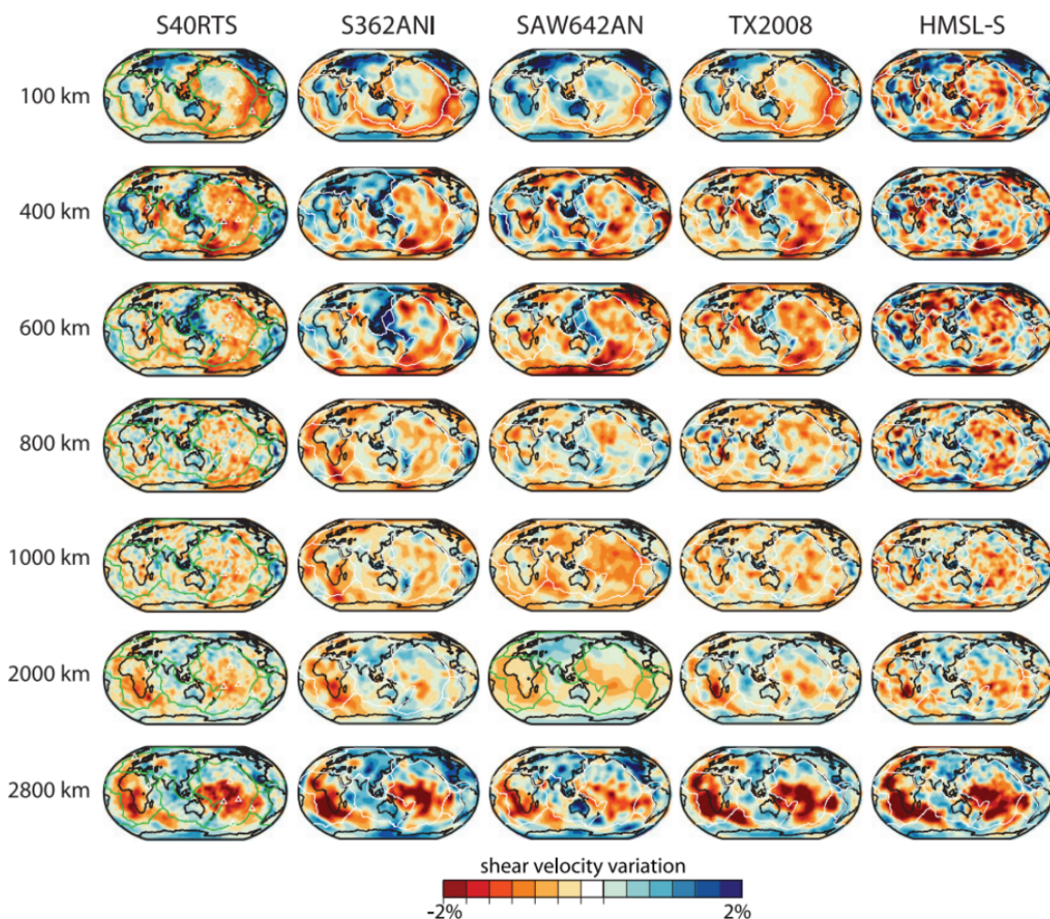
Fig. 9: Depth slices from a range of different S-wave tomographic models, taken from Ritsema et al. (2011). In all cases the Pacific and African LLSVPs can be seen at the base of the mantle. The dynamical significance of these features remains unclear.
