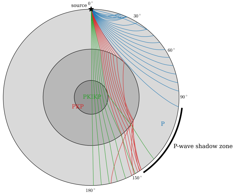
Fig. 3: P-wave ray paths within the earth model PREM for a source at the surface, calculated using the ray equations of this lecture. Rays that turn within the mantle (blue) emerge at epicentral angles up to about 98^\circ . PKP rays (red), which turn within the outer core, emerge beyond about 145^\circ , while PKIKP rays (green), which pass through the inner core, can emerge within the shadow zone. The sudden reduction in P-wave velocity on entering the fluid outer core thus leads to the so-called “P-wave shadow zone”, while no S-waves are able to propagate within the outer core at all.
