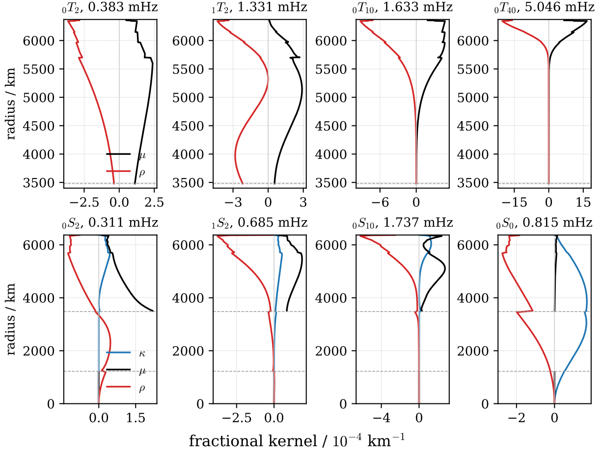
Fig. 7: Sensitivity kernels of the toroidal (upper row) and spheroidal (lower row) modes of Fig. 3. The kernels are shown in fractional form, so that \delta\omega_k/\omega_k = \int_0^b (\tilde{K}_\kappa \delta\kappa/\kappa + \tilde{K}_\mu \delta\mu/\mu + \tilde{K}_\rho \delta\rho/\rho) dr . The toroidal kernels follow from eq. (30); the spheroidal ones, which include the effects of self-gravitation, were obtained numerically. The density kernel of 0S_2 changes sign in the outer core, gravity and inertia competing for this gravest mode.
