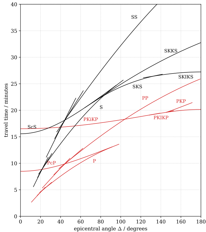
Fig. 4: Travel time curves for the main body-wave phases within the earth model PREM, for a source at the surface, calculated using the ray equations of this lecture (phases travelling as P-waves in the mantle in red, and as S-waves in black). Only rays whose turning or reflection point lies below 220 km depth are shown. The nomenclature for the different phases can be ignored.
