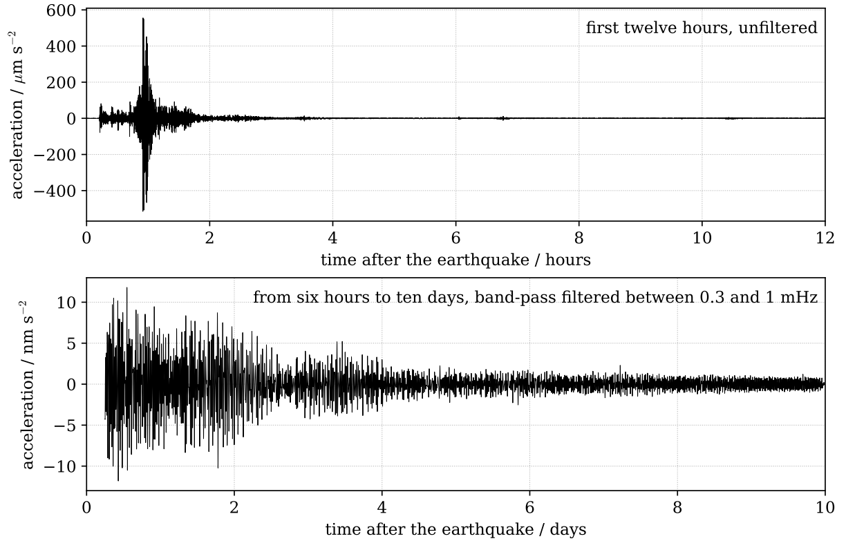
Fig. 1: Vertical-component acceleration recorded at the Black Forest Observatory in Germany following the 2011 Tohoku earthquake in Japan (moment magnitude 9.1). The amplitude spectra corresponding to Fig upper panel shows the first twelve hours of the record, dominated by the surface waves, which circle the Earth several times. 1. In some cases individual mode peaks can be identified The lower panel shows the record from six hours to ten days after the earthquake, but especially at higher-frequencies there is substantial overlap of band-pass filtered between 0.3 and 1 mHz to isolate the peaks lowest-frequency free oscillations. Their amplitude decays in a roughly exponential fashion over several days. This decay is due both to attenuation and an insufficiently long time series within the Earth, but we ignore this effect within our current discussion.
