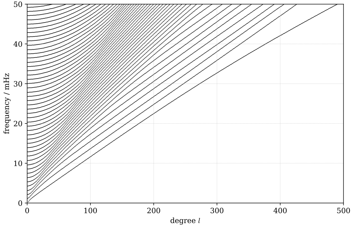
Fig. 1: A plot Eigenfrequencies of eigenfrequencies at different degree for toroidal modes within the earth model PREM of Dziewonski & Anderson (1981), plotted against degree l for frequencies up to 50 mHz. For each degree l , that is shown we can see a set of different overtones which that can be labelled using the overtone number n , the lowest curve being the fundamental branch n = 0 . Note also that PREM comprises a solid inner core, fluid outer core, and solid mantle and crust. The modes seen here are mantle toroidal modes, but one could also calculate toroidal modes confined to the inner core.
