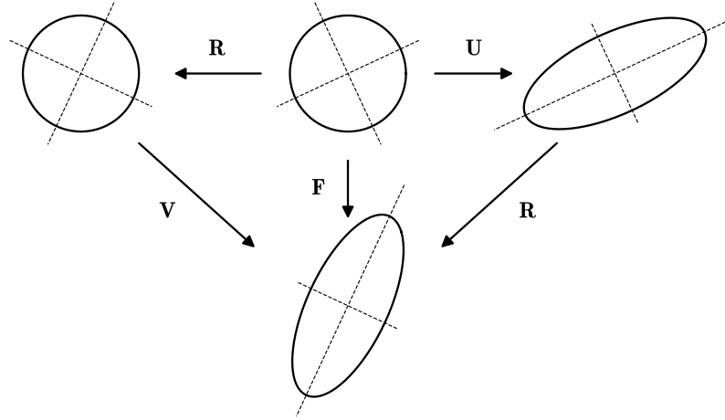
Fig. 1: Under an invertible matrix F , a circle (in three dimensions, a sphere) is mapped to an ellipse (ellipsoid) . Using this fact, the geometric meaning of the polar decomposition theorem is shown. An undeformed circle is shown in the centre of the upper row, with the dashed lines along the eigenvectors of the symmetric matrix U ; in the other panels the dashed lines show the images of these axes.
