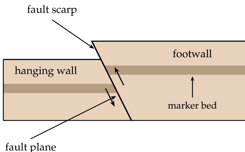
Fig. 1: A schematic diagram of cross-section through a normal fault. You do not need to learn the associated terminology.
