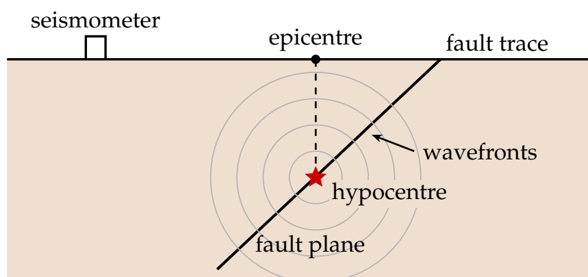
Fig. 1: A diagram showing an idealised planar fault. The hypocentre is the point on the fault where rupture initiates, while the epicentre is simply the projection of this point onto the Earth's surface. It is the hypocentre location that can be estimated by looking at the arrival times of high-frequency seismic waves recorded on seismometers.
