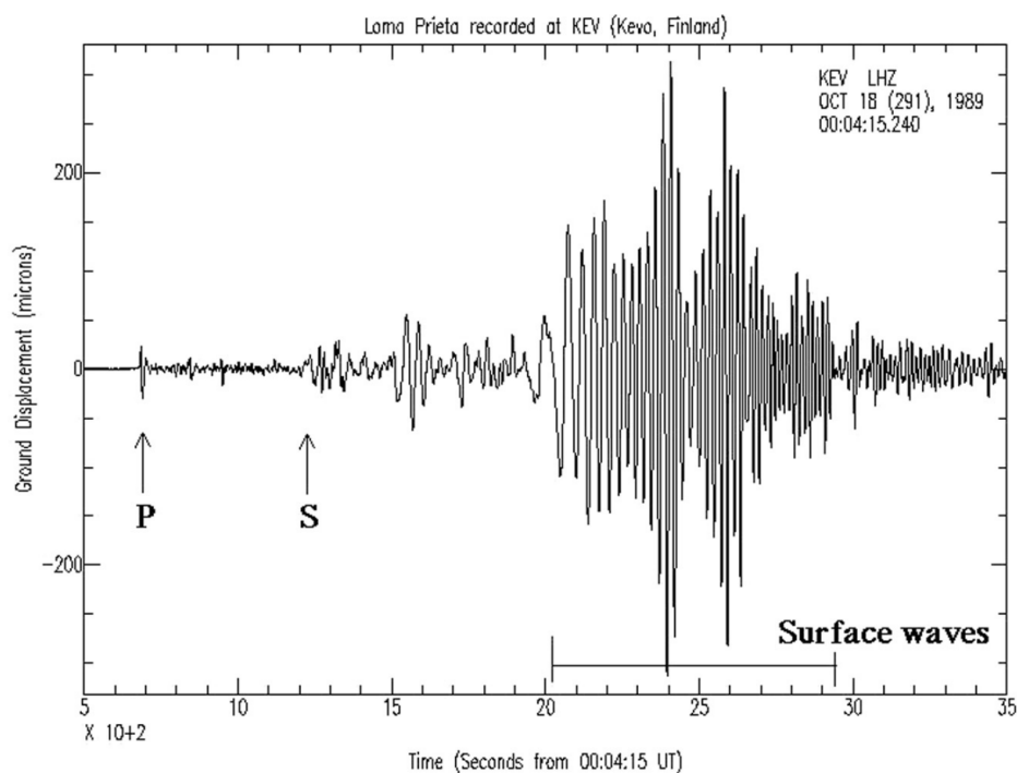
Fig. 2: A vertical component seismogram recorded in Finland following an earthquake in California ( the 1989 Loma Prieta earthquake recorded at station KEV ). The P-wave arrival can be seen very clearly, while later arriving phases are significantly harder to identify.
