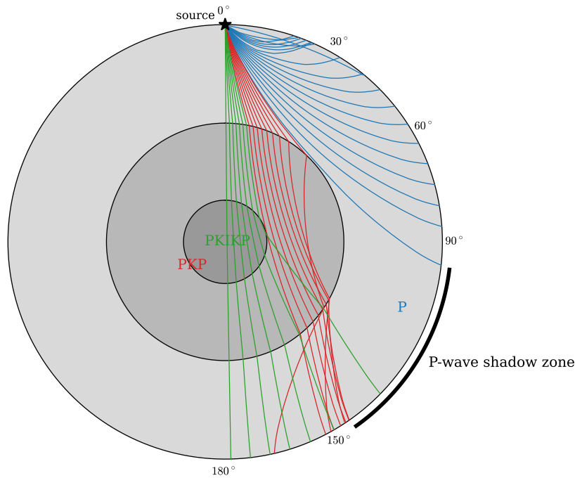
Fig. 3: A diagram showing some of the many possible P-wave ray paths within the Earth model PREM for a source at the surface, calculated using the ray equations of this lecture. Note in particular Rays that turn within the mantle (blue) emerge at epicentral angles up to about 98°. PKP rays (red), which turn within the outer core, emerge beyond about 145°, while PKIKP rays (green), which pass through the inner core, can emerge within the shadow zone. The sudden reduction in P-wave velocity when on entering the fluid outer core thus leads to the so-called “P-wave shadow zone”, while no S-waves are able to propagate within this region the outer core at all.
