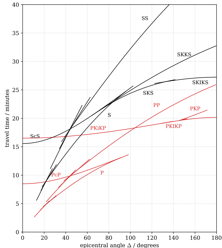
Fig. 4: Travel time curves determined for the main body-wave phases within the earth model PREM, for a large number source at the surface, calculated using the ray equations of seismic this lecture (phases within travelling as P-waves in the Earth mantle in red, and as S-waves in black). Only rays whose turning or reflection point lies below 220 km depth are shown. The nomenclature for the different phases can be ignored.
