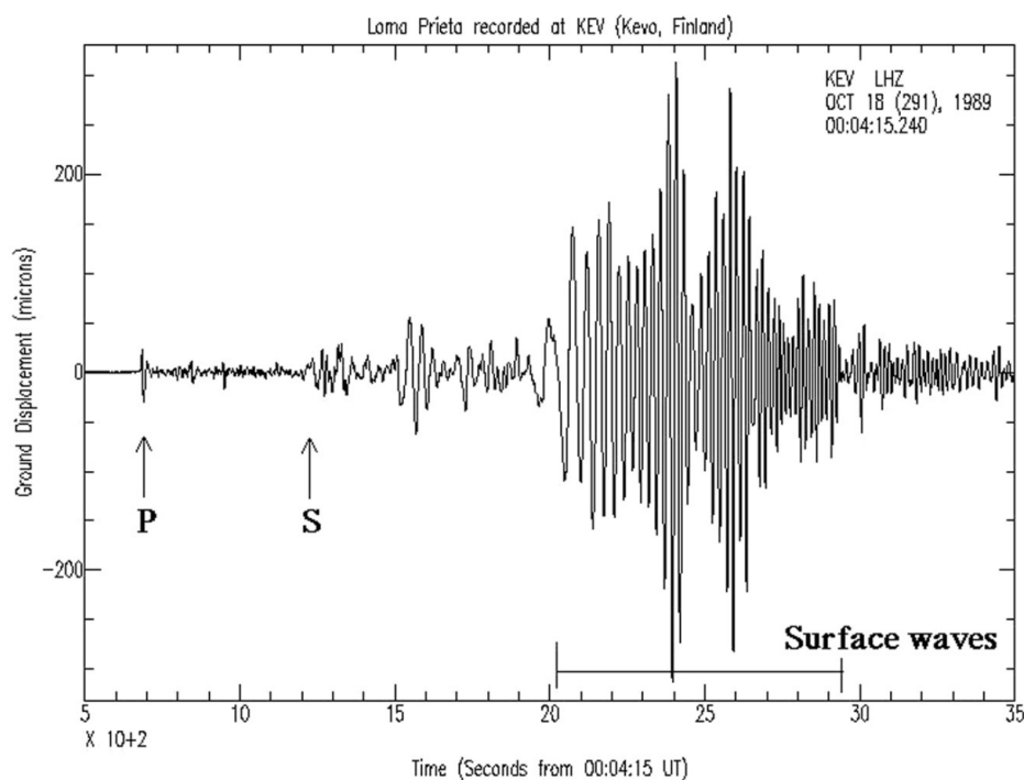
Fig. 2: A vertical component seismogram recorded in Finland following an earthquake in California (the 1989 Loma Prieta earthquake recorded at station KEV). The P-wave arrival can be seen very clearly, while later arriving phases are significantly harder to identify.
