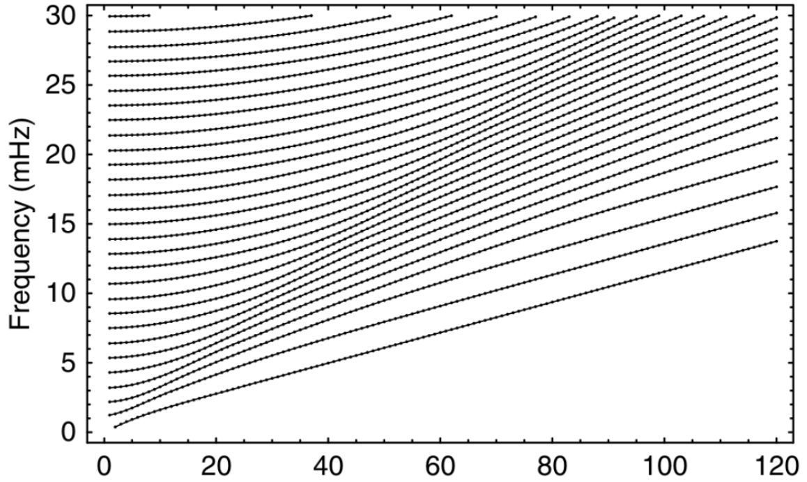
Fig. 1: A plot of eigenfrequencies at different degree degrees for toroidal modes within the earth model PREM of Dziewonski & Anderson (1981). For each degree, l , that is shown we can see a set of different overtones which can be labelled using the overtone number, n . Note also that PREM comprises a solid inner core, fluid outer core, and solid mantle and crust. The modes seen here are mantle toroidal modes, but one could also calculate toroidal modes confined to the inner core.
