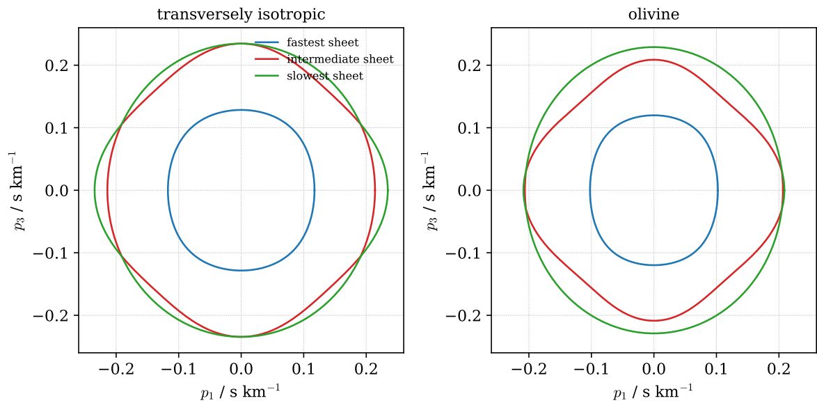
Fig. 1: Plane sections through the slowness surface associated with surfaces of two randomly selected anisotropic elastic materials, calculated numerically from the Christoffel equation . On the left is a transversely isotropic medium, with the section containing the symmetry axis (which is vertical); on the right is a single crystal of olivine, an orthorhombic mineral that makes up much of the upper mantle, using the elastic constants of Abramson et al. (1997). The three sheets of the slowness surface are shown in different colours, and there are directions along which two of the sheets touch .
