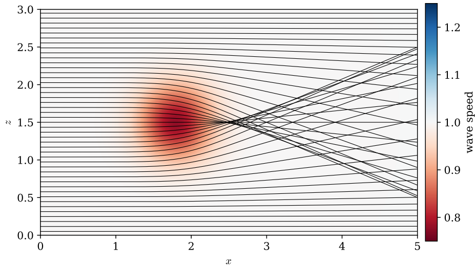
Fig. 3: An example of ray tracing within Rays from an initially plane wavefront passing through a heterogeneous body smooth region of low wave speed, and obtained by numerical integration of Hamilton's equations. Behind the formation of anomaly the rays cross, and their envelope forms a caustic due to an area of low velocity .
