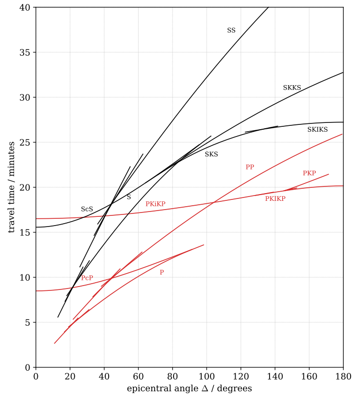
Fig. 4: Travel time Travel-time curves determined for the main body-wave phases within the earth model PREM, for a large-number source at the surface, calculated using the ray equations of seismic this lecture (phases within travelling as P-waves in the Earthmantle in red, and as S-waves in black). Only rays turning below a depth of 220 km are shown. The nomenclature for the different phases can be ignored.
