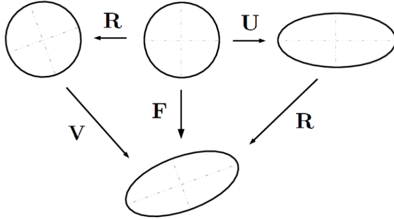
Fig. 1: Under an invertible matrix F , a sphere is mapped to an ellipsoid. Using this fact, the geometric meaning of the polar decomposition theorem is shown. An undeformed circle is shown in the centre of the upper row, with the dashed lines along the eigenvectors of the symmetric matrix U .
