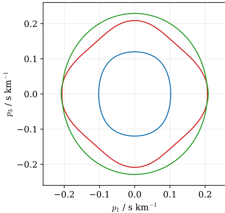
olivine
