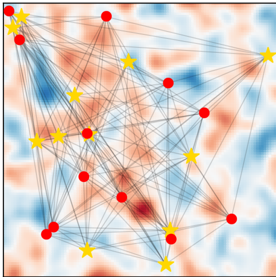
true model
