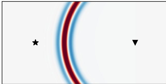
adjoint field \nabla \cdot \mathbf{u}'
