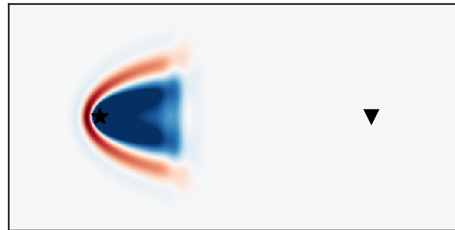
kernel K_\alpha accumulated so far
