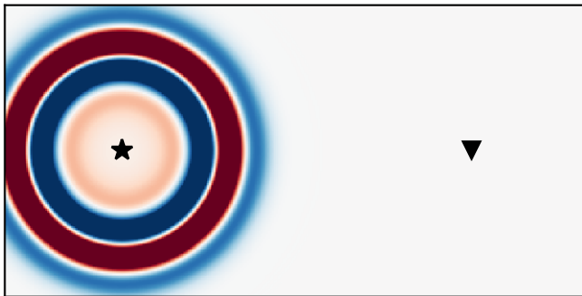
forward field \nabla \cdot \mathbf{u}
