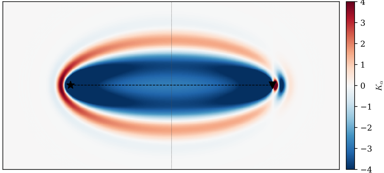
kernel K_\alpha
