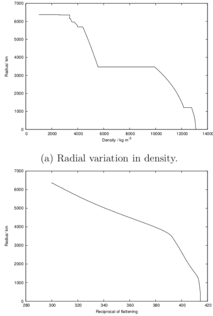
Fig. 1: The upper panel shows variations in the Earth's spherically averaged density structure as determined from free oscillation data along with mass and moment of inertia constraints. The lower panel then plots the reciprocal of the ellipticity as determined through numerical solution of Clairaut's equation.
