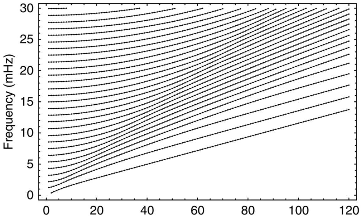
Fig. 1: A plot of eigenfrequencies at different degrees for toroidal modes within the earth model PREM of Dziewonski & Anderson (1981). For each degree, l , that is shown we can see a set of different overtones which can be labelled using the overtone number, n . Note also that PREM comprises a solid inner core, fluid outer core, and solid mantle and crust. The modes seen here are mantle toroidal modes, but one could also calculate toroidal modes confined to the inner core.
