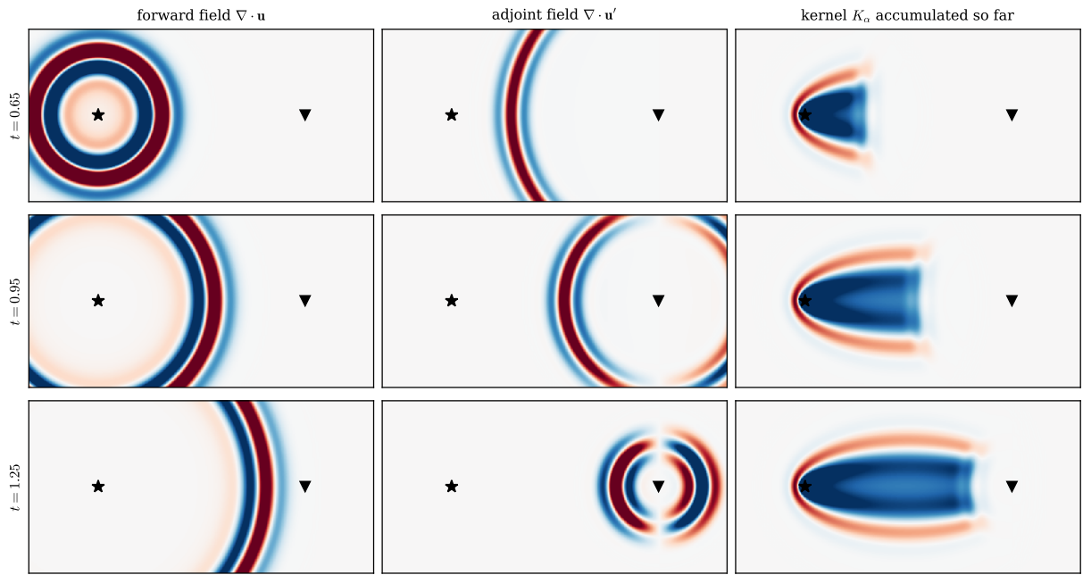
Fig. 3: Construction of a cross-correlation delay-time kernel by the adjoint method in a two-dimensional homogeneous body. The star marks an explosive source and the triangle a receiver. Each row shows one instant: the divergence of the forward field (left), the divergence of the adjoint field, which is driven at the receiver and satisfies terminal conditions, so that it spreads outwards as time runs backwards (centre), and the kernel K_\alpha accumulated up to that instant (right). The kernel grows only where the two fields overlap.
