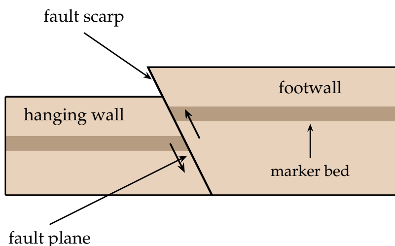
Fig. 1: A schematic diagram of a fault. You do not need to learn the associated terminology.
