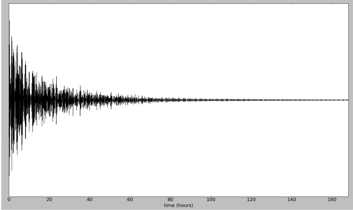
Fig. 1: A seven-day-long vertical-component seismogram following the magnitude 8.2 earthquake in Bolivia in 1994. Note that the overall amplitude decays in a roughly exponential fashion. This is due to attenuation within the Earth, but we ignore this effect within our current discussion.
