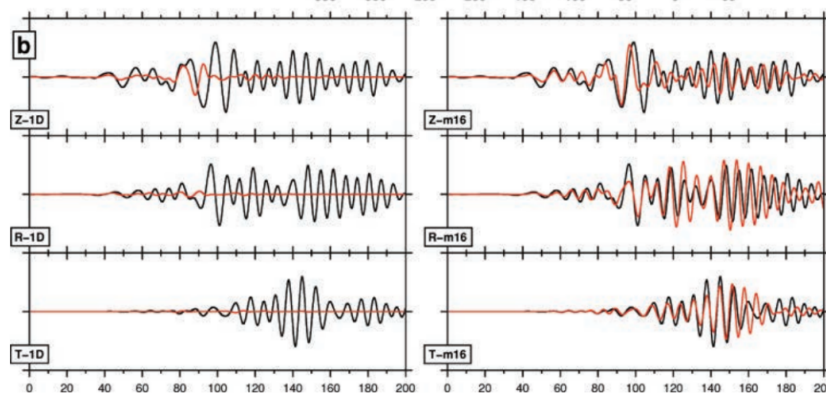
Fig. 2: An example of observed and synthetic three-component seismograms from a waveform tomographic study of Southern California. Data are shown in black, and synthetics in red. On the left the comparison is made prior to inversion, with the synthetics calculated in a laterally homogeneous model. The right-hand side then shows the data fit following inversion involving 16 iterative model updates. Taken from Tape et al. (2010).
