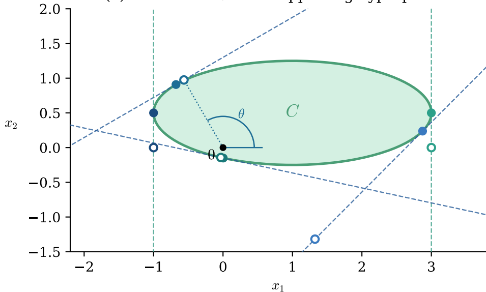
(a) Convex set C with supporting hyperplanes
