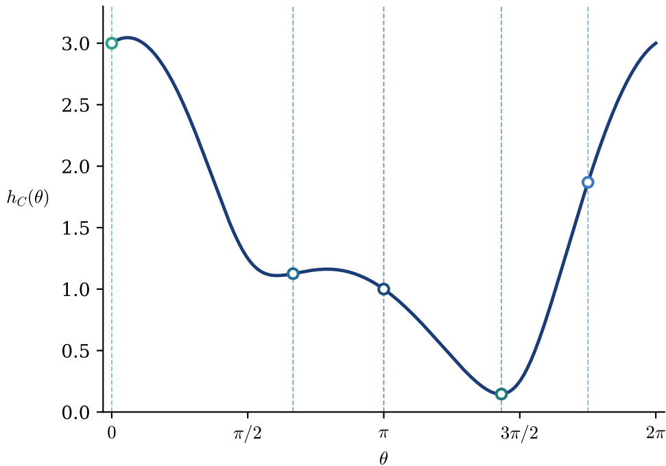
(b) Support function h_C(\theta)
