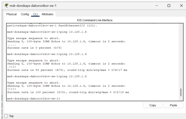
Figure 14: ping
