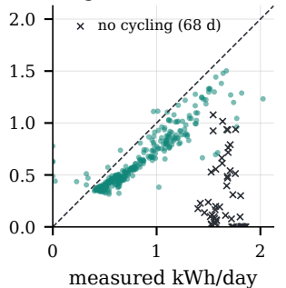
Fridge ( r = 0.90 excl. x)
