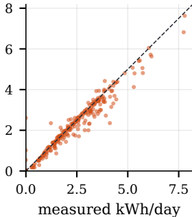
Water heater ( r = 0.98 , 404 days)
