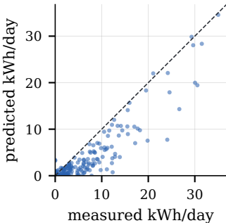
Air conditioner ( r = 0.92 , 404 days)
