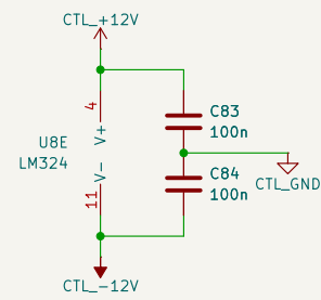
U8: LM324, LED drivers
