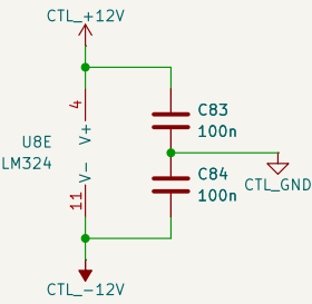
U8: LM324, LED drivers
