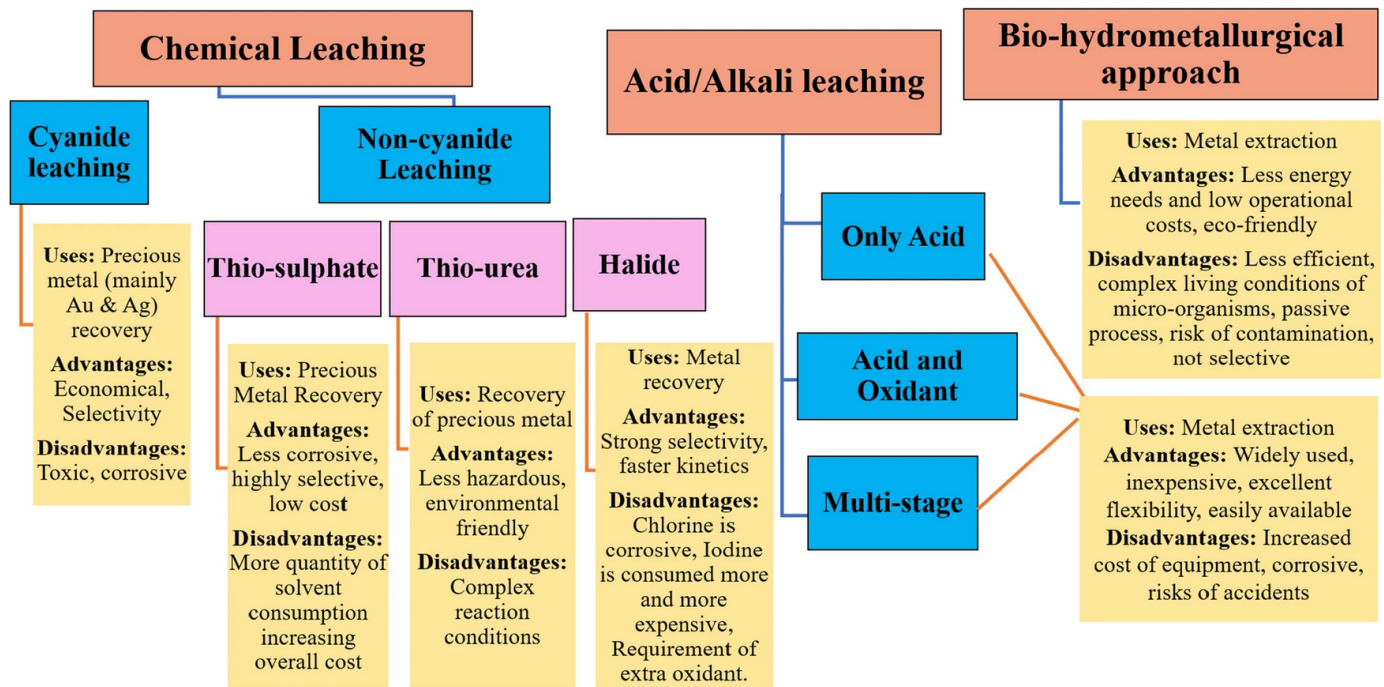
Fig. 2. Overview of the different hydrometallurgical processes. Source javed2024 .
