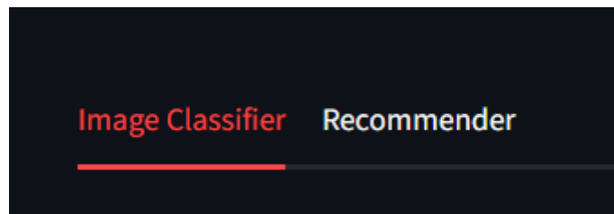
Figure 1.1: NavigationMenu
