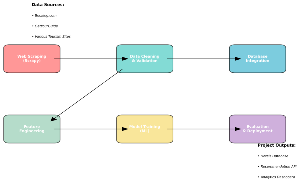
Figure 1.3: TravelHunters Data Science Pipeline
