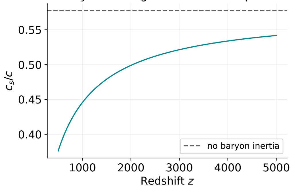
Baryon loading reduces sound speed
