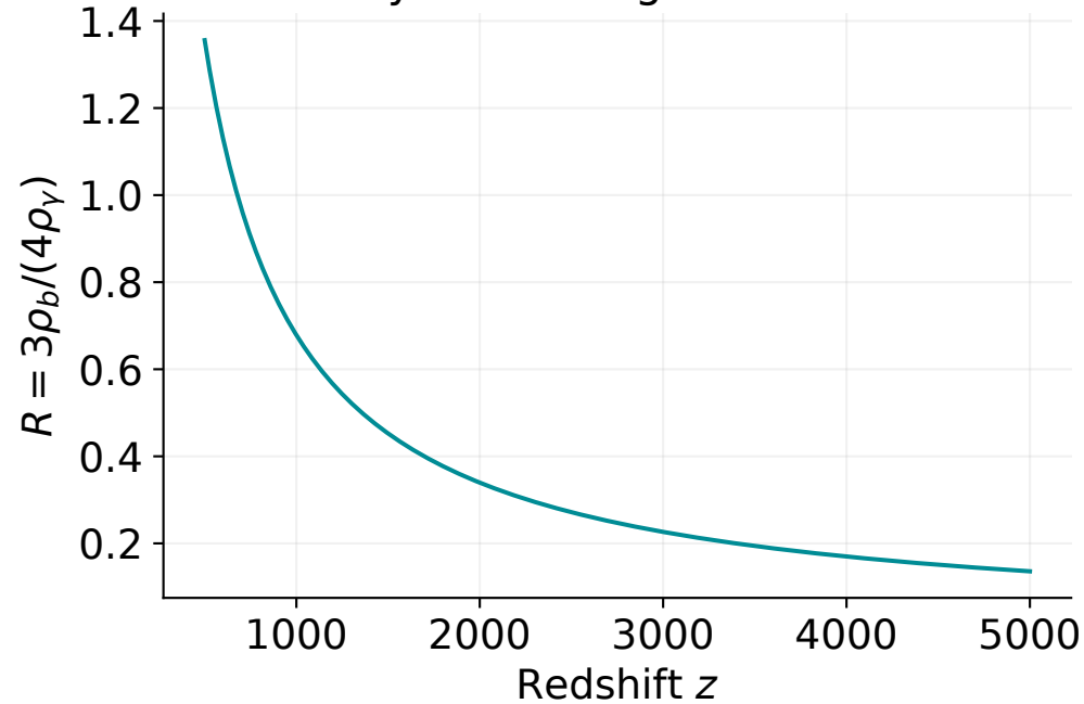
Relative baryon inertia grows as redshift falls
