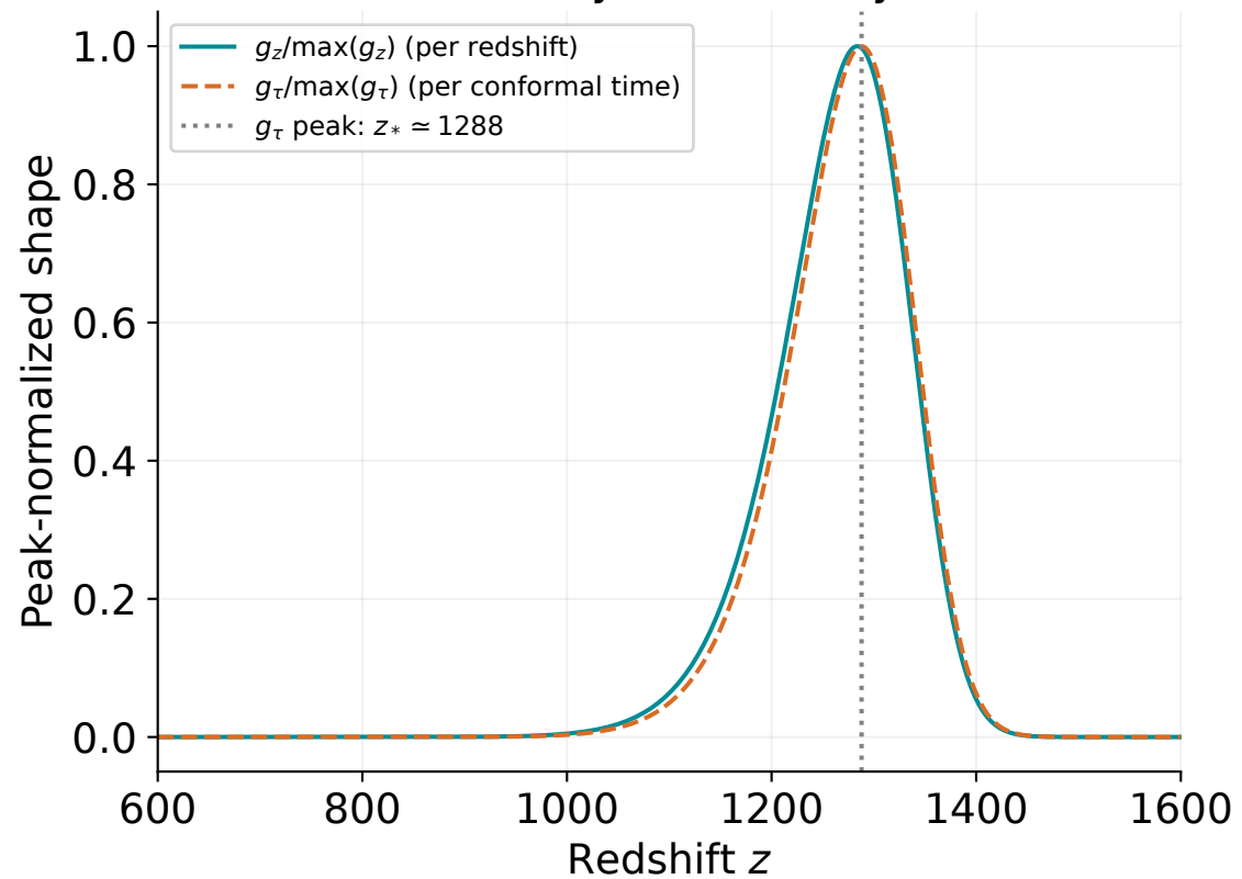
Saha-model visibility: two density conventions
