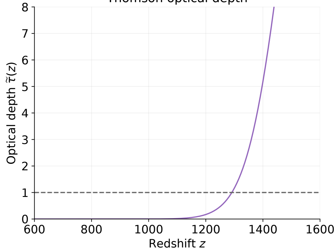
Thomson optical depth
