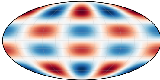
\text{Re } Y_{5,2}
