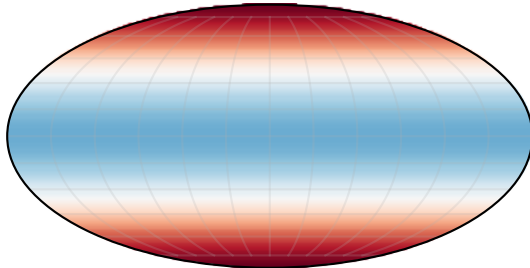
\text{Re } Y_{2,0}
