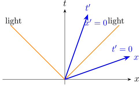
Figure 1: A qualitative two-observer diagram in units with c = 1 . The primed axes are a coordinate grid for the moving frame; no tick marks or interval construction are needed yet.
