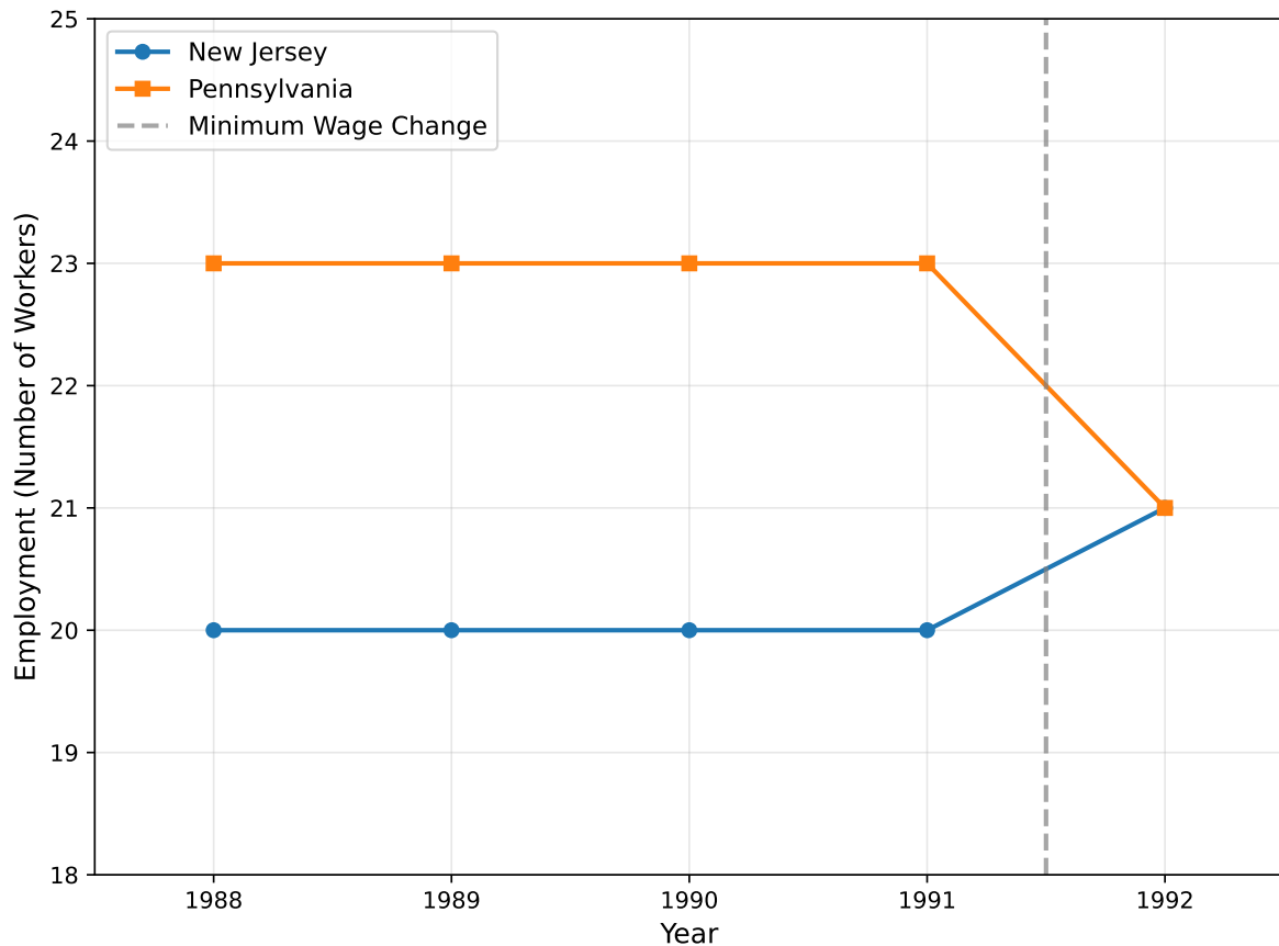
Figure 3.8: Hypothetical example with stable pre-trends (1988-1991)
