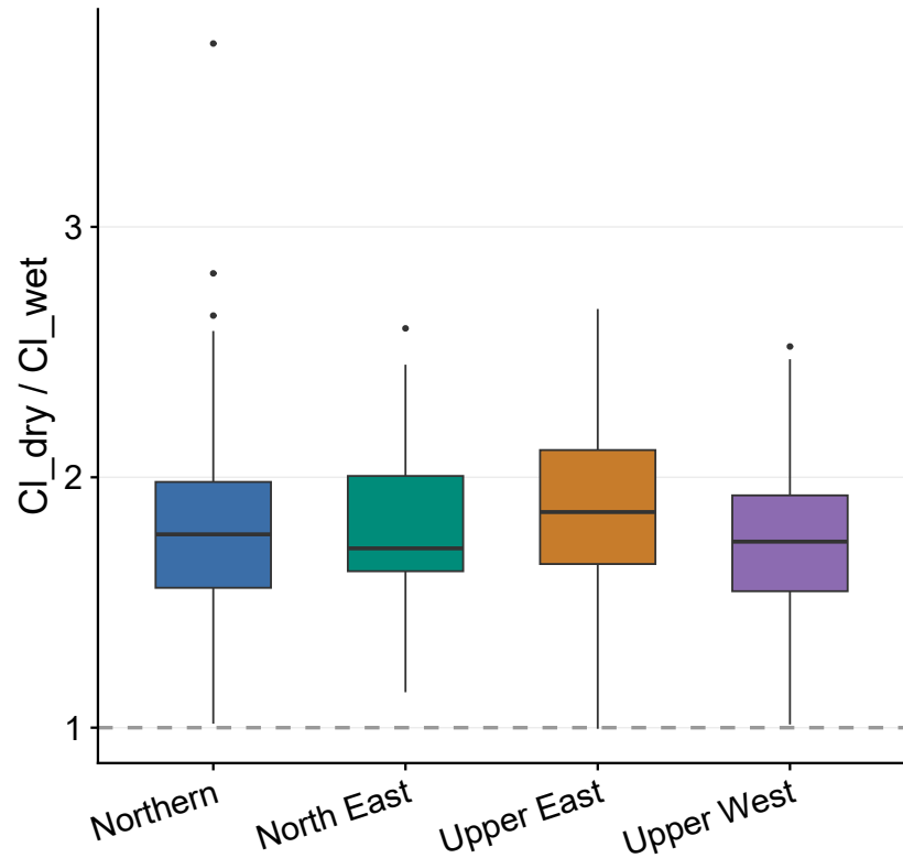
a Dry/wet evapoconcentration (CI-based)
