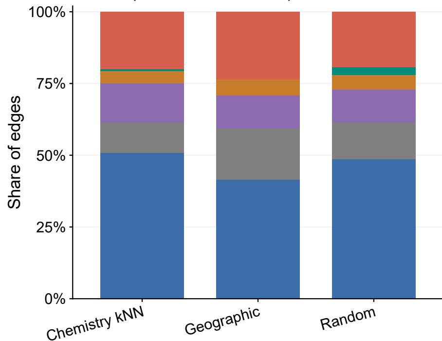
a Inferred process-network composition
