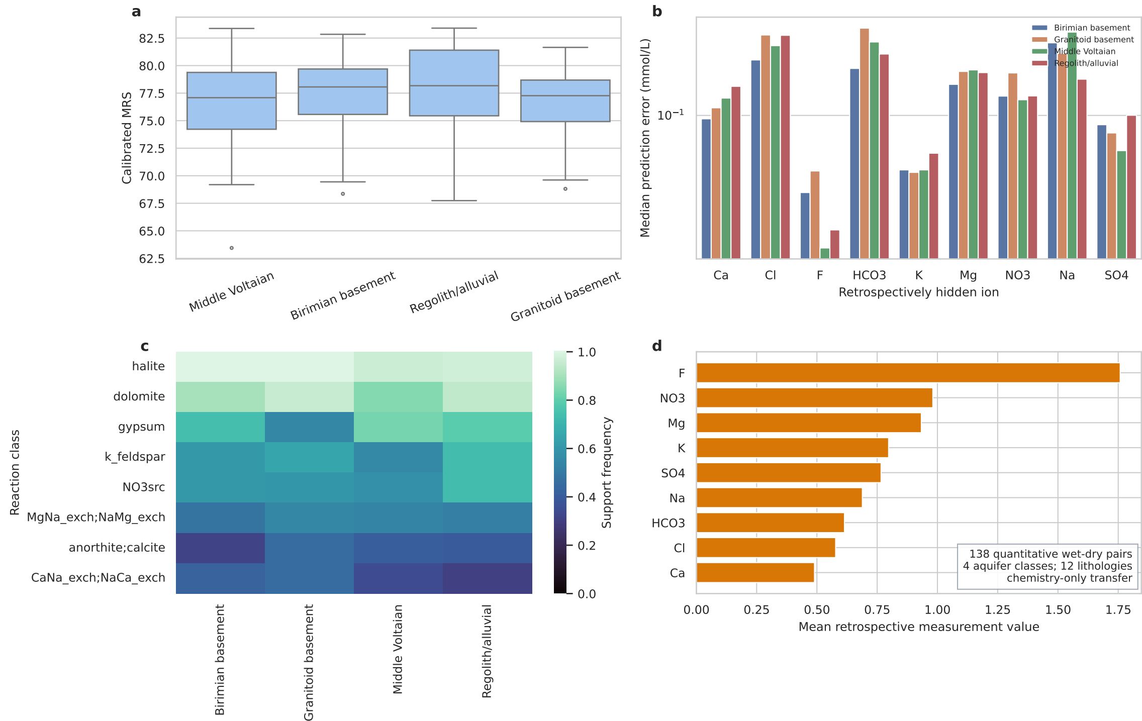
Figure 6 | Northern Ghana seasonal chemistry remains only partially identifiable
