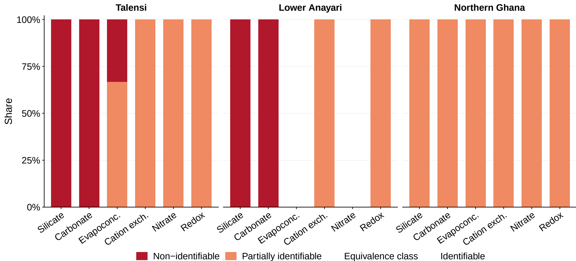
Figure S10. Identifiability composition per process family and dataset
