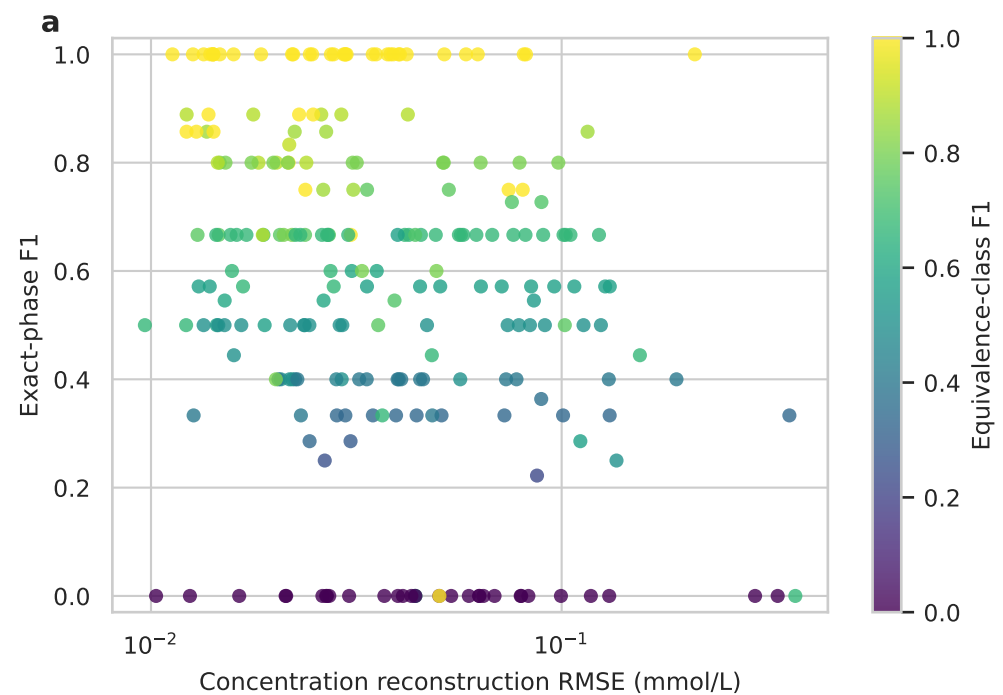
Figure 2 | Accurate concentration fits can conceal incorrect pathways
