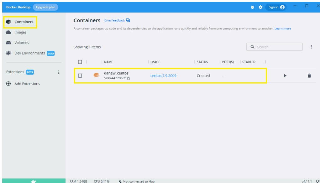
Docker Desktop
