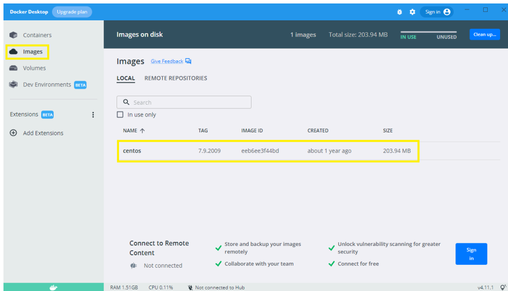
Docker Desktop
