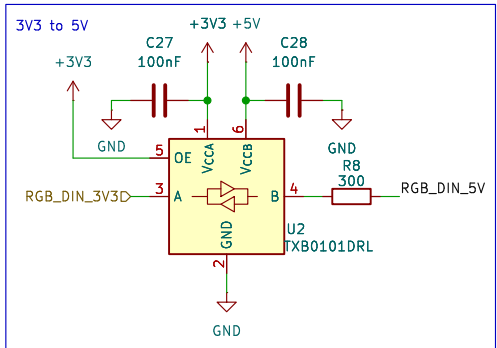
LED Level Shifter
