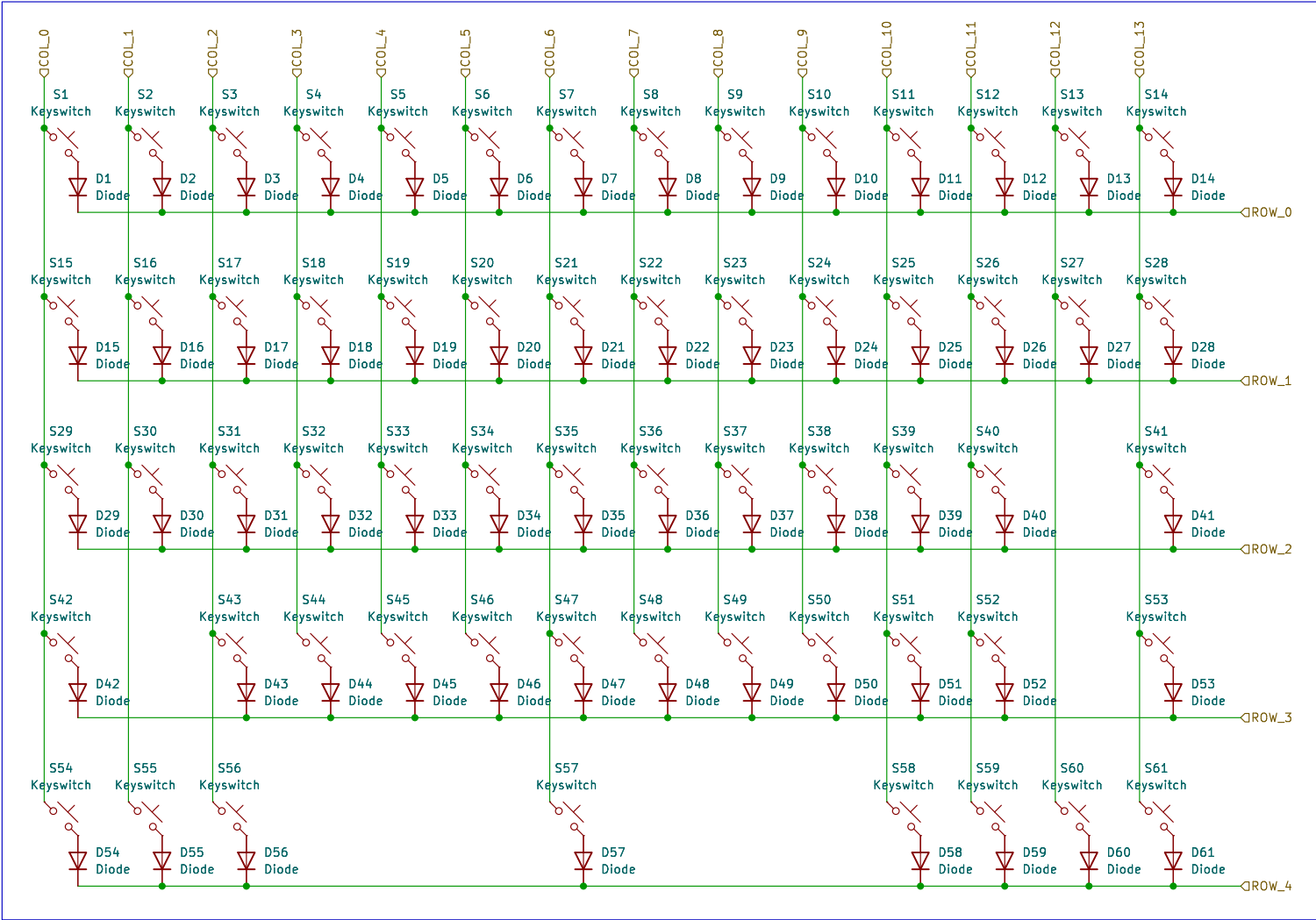
Key Switch Matrix
