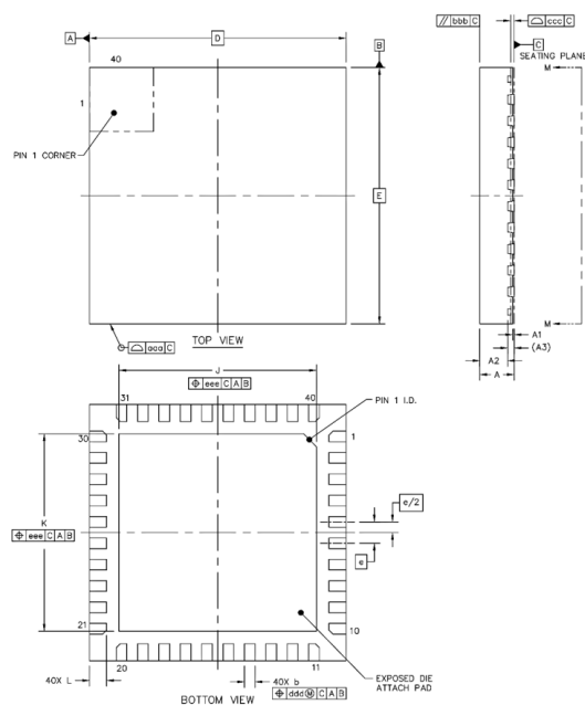
QFN40, 6mm x 6mm, 0.5mm pitch
