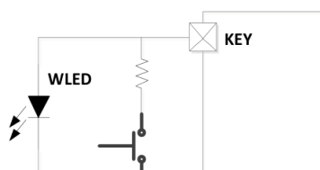
Figure 3 Key (button) wiring
