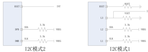
I2C Mode 2 (left) and I2C Mode 1 (right)
