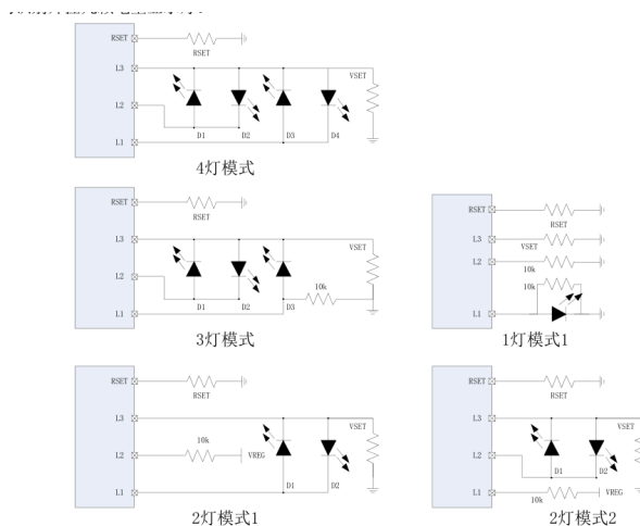
Figure 4 Pin connections for 4-LED, 3-LED, 2-LED, and 1-LED display modes
