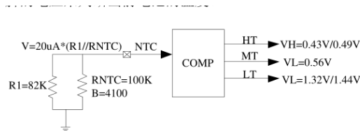
Figure 5 Battery NTC comparator
