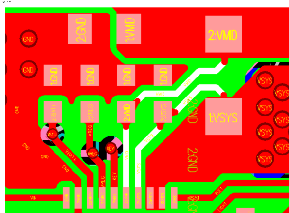
10 mΩ sense-resistor routing example
