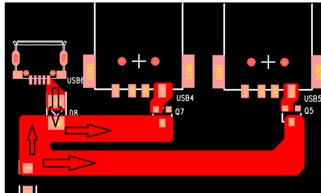
Routing from the sense resistor to the output MOSFETs
