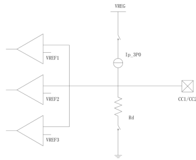
USB-C CC pull-up / pull-down network
