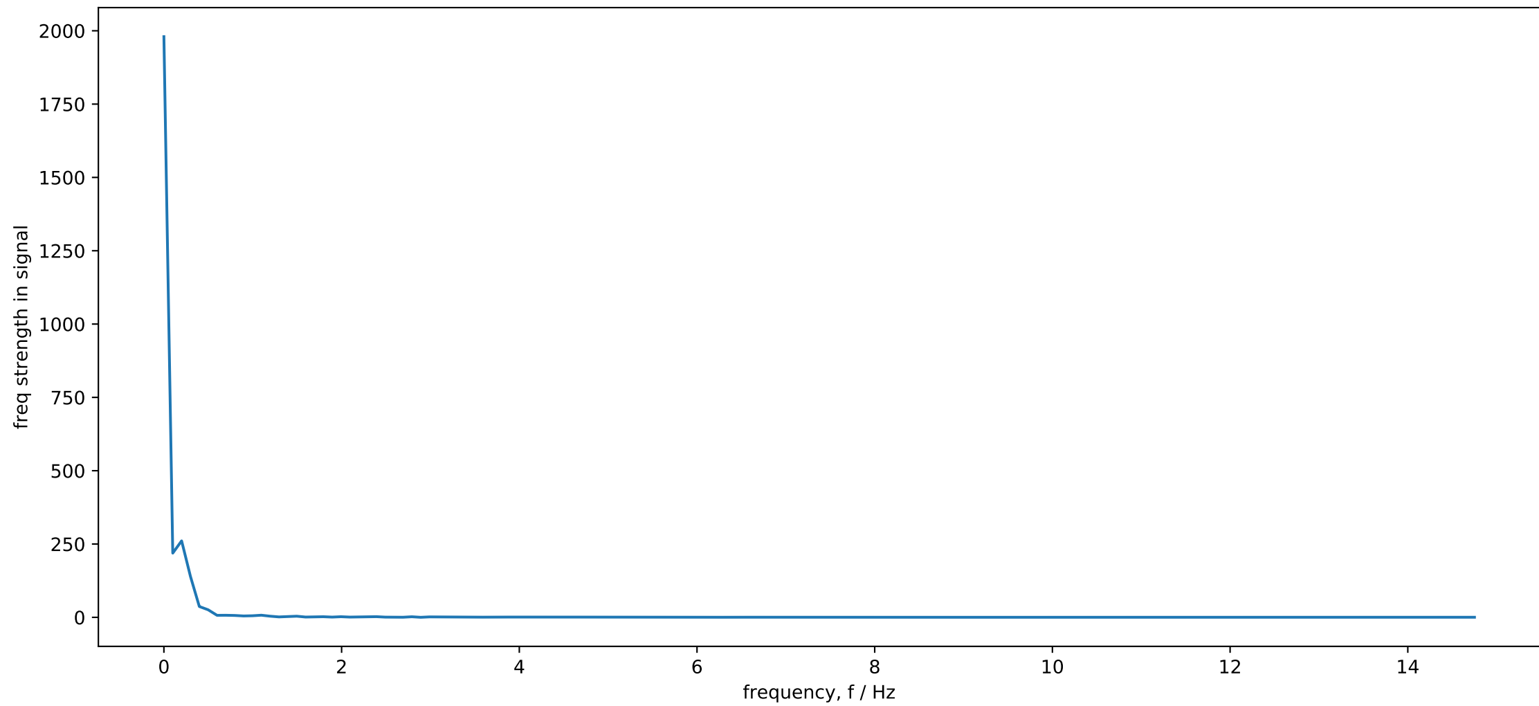
discrete FFT
